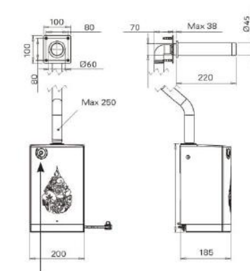
Airflow intensity adjustment button
